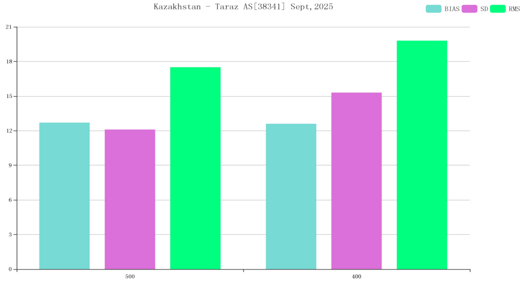
Figure 31 BIAS、SD and RMS of WIN_D for station 38341*(OBS-TIME:12)
