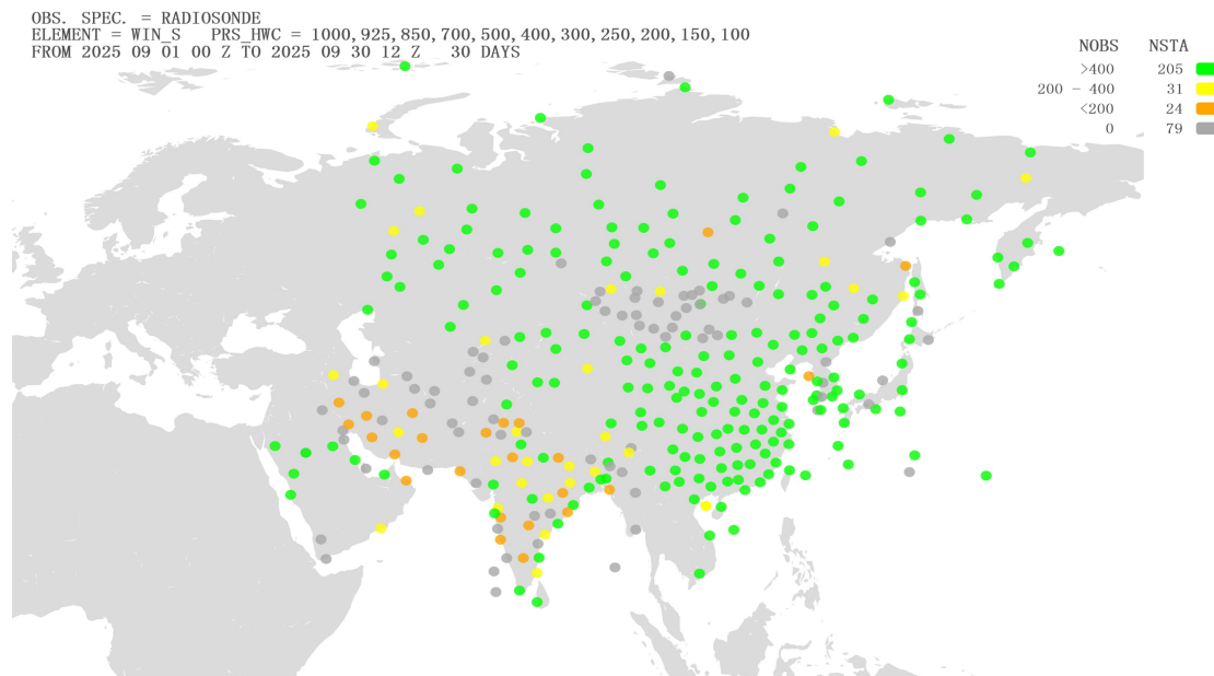
Figure 21 Location of all radiosonde stations reporting vector wind observations in Region II over the month of September 2025. NOBS shows the total number of observations received at RWC-Beijing, corresponding total number of stations (NSTA) and color scale are shown at the top of the figure, color green refers to NOBS is higher than 400, color yellow refers to NOBS is between 200 and 400(including 400), color orange refers to NOBS is between 0 and 200(including 200), and color gray refers to NOBS is 0
