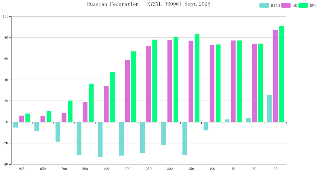
Figure 9 BIAS、SD and RMS of GPH for station 36096*(OBS-TIME:00)
