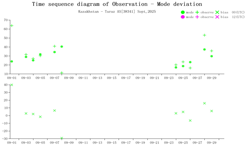
Figure 26 Time-series representation of WIN_S Obs minus first guess for station 38341*(Level:200)
