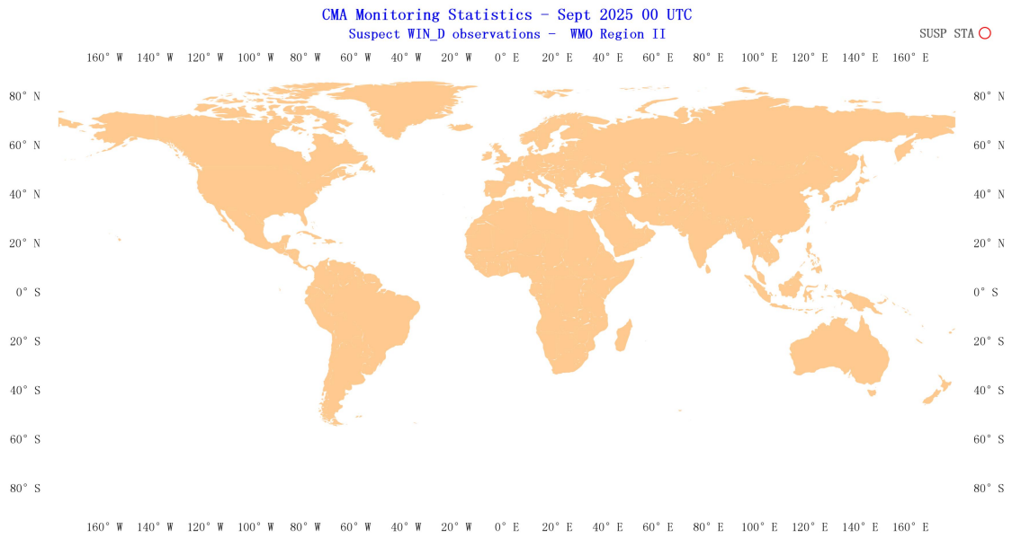
Figure 29 Distribution of suspect stations - Wind Direction 00 UTC
