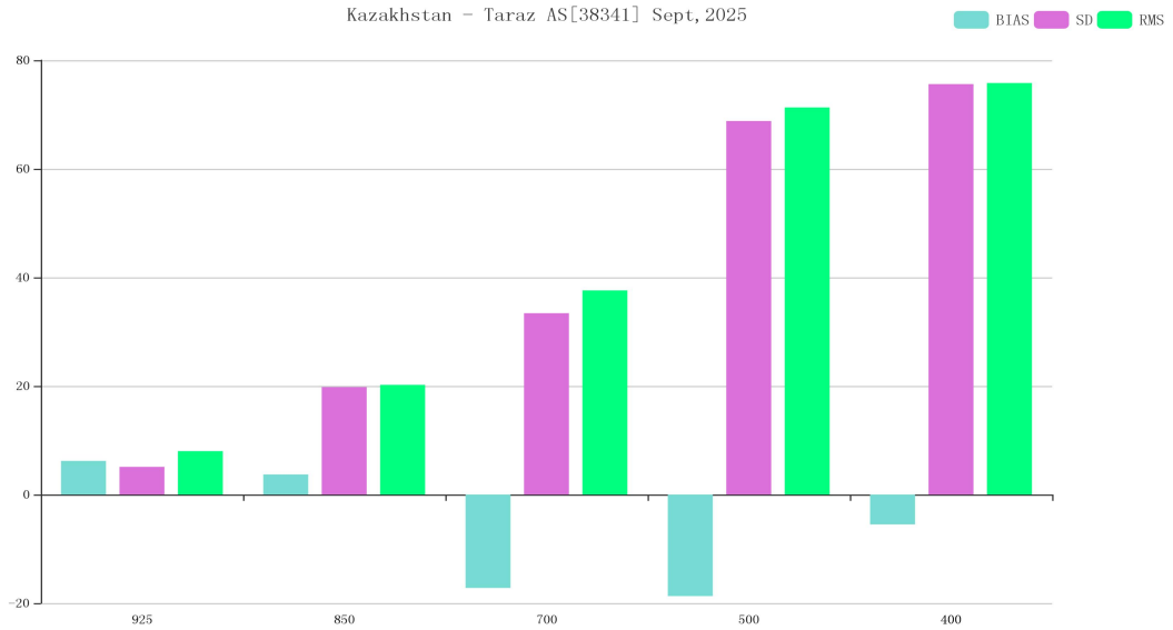
Figure 11 BIAS、SD and RMS of GPH for station 38341*(OBS-TIME:00)
