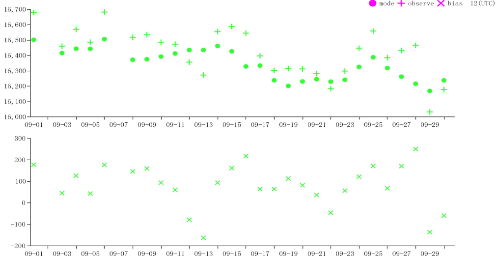
Figure 6 Time-series representation of GPH Obs minus first guess for station 31770*(Level:100)
