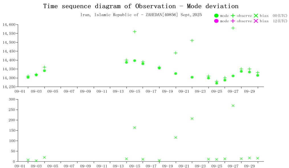
Figure 16 Time-series representation of GPH Obs minus first guess for station 40856*(Level:150)
