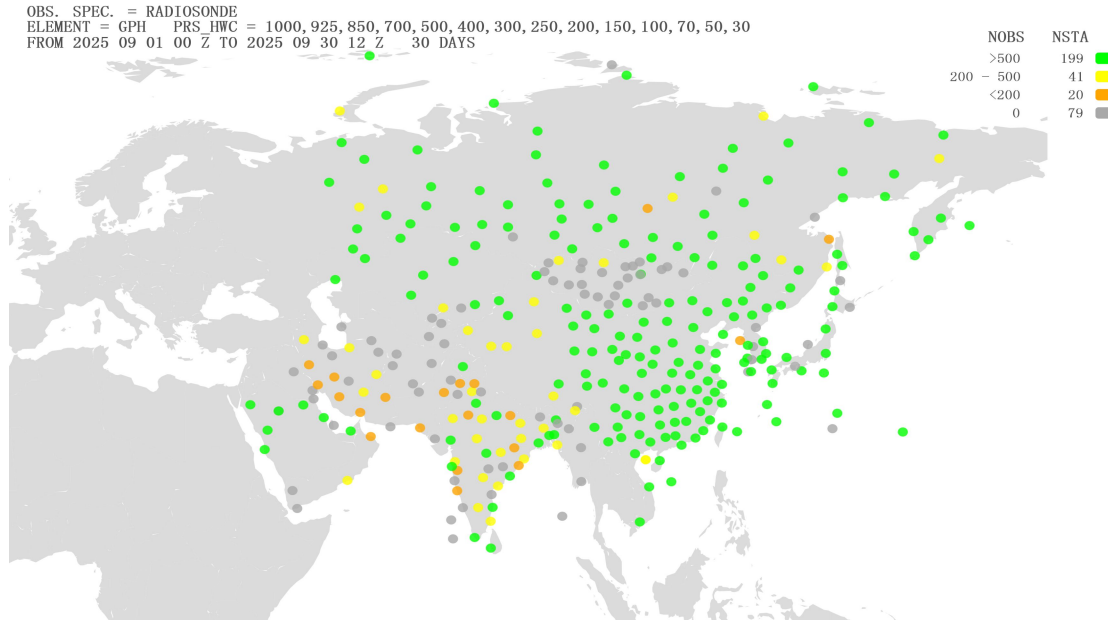
Figure 1 Location of all radiosonde stations reporting geopotential height observations in Region II over the month of September 2025. NOBS shows the total number of observations received at RWC-Beijing, corresponding total number of stations (NSTA) and color scale are shown at the top of the figure, color green refers to NOBS is higher than 500, color yellow refers to NOBS is between 200 and 500(including 500), color orange refers to NOBS is between 0 and 200(including 200), and color gray refers to NOBS is 0
