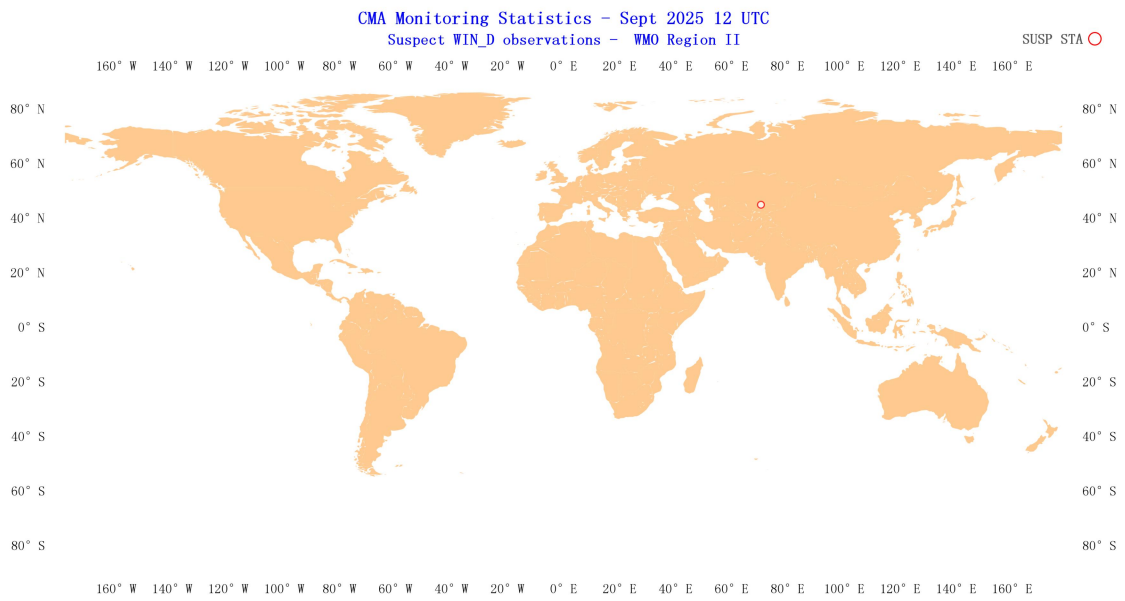
Figure 30 Distribution of suspect stations - Wind Direction 12 UTC
