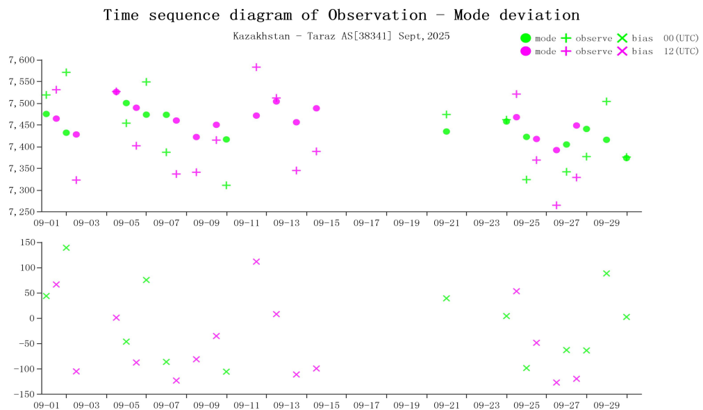
Figure 12 Time-series representation of GPH Obs minus first guess for station 38341*(Level:400)
