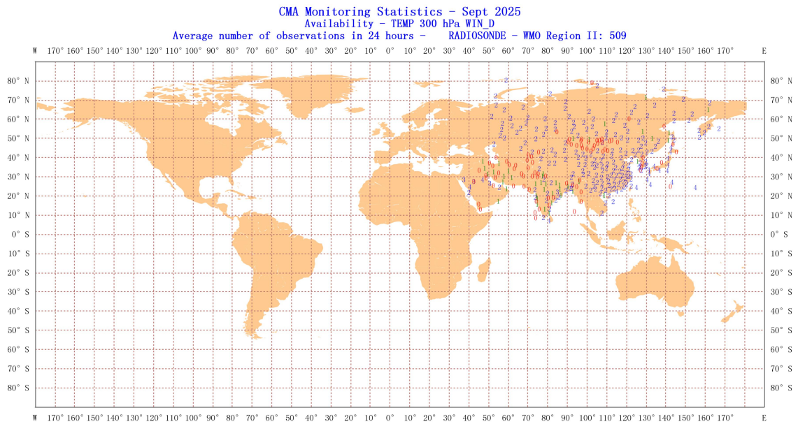
Figure 28 Location of all radiosonde stations reporting wind direction average number of observations in 24 hours in Region II over the month of September 2025
