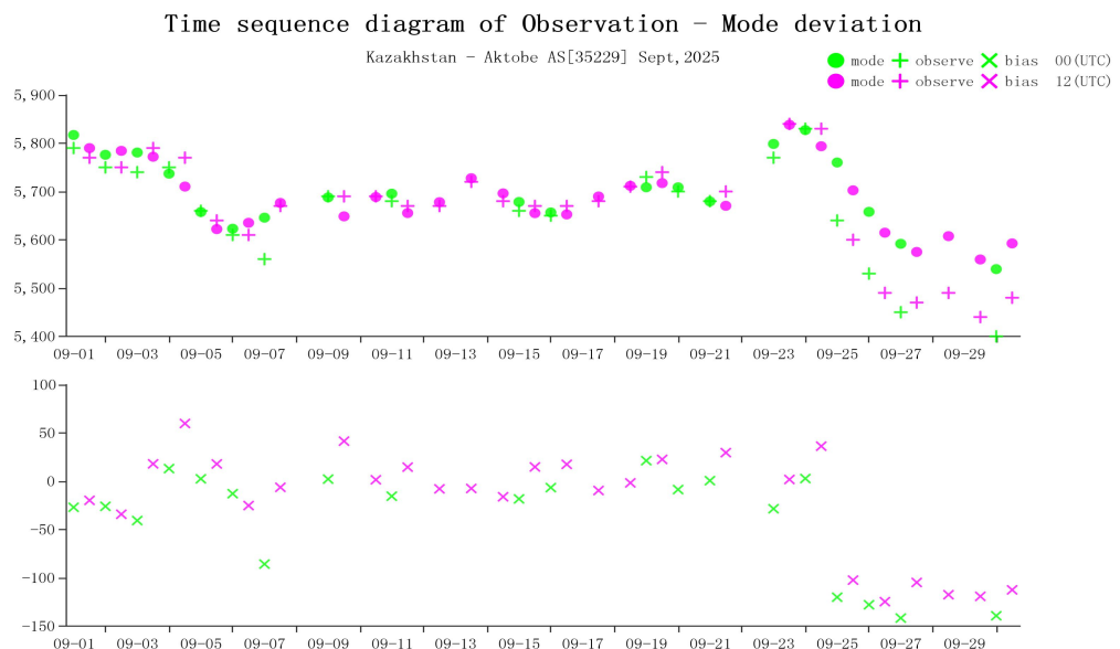
Figure 8 Time-series representation of GPH Obs minus first guess for station 35229*(Level:500)
