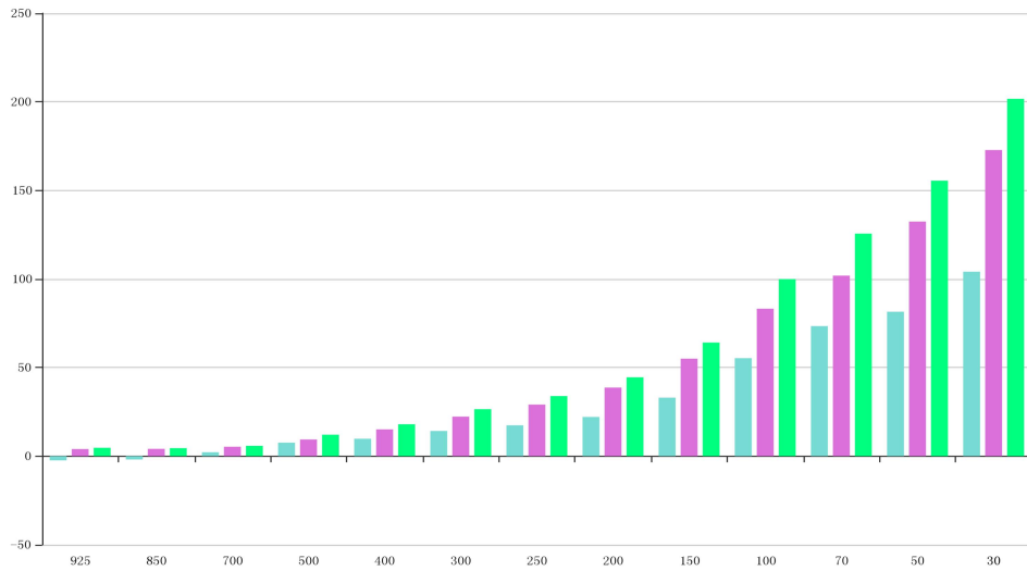
Figure 19 BIAS、SD and RMS of GPH for station 58027(OBS-TIME:00)
