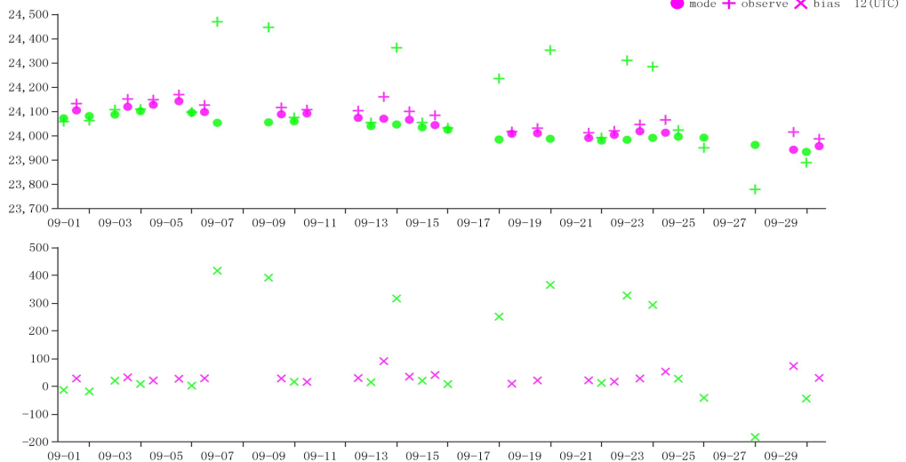
Figure 20 Time-series representation of GPH Obs minus first guess for station 58027(Level:30)
