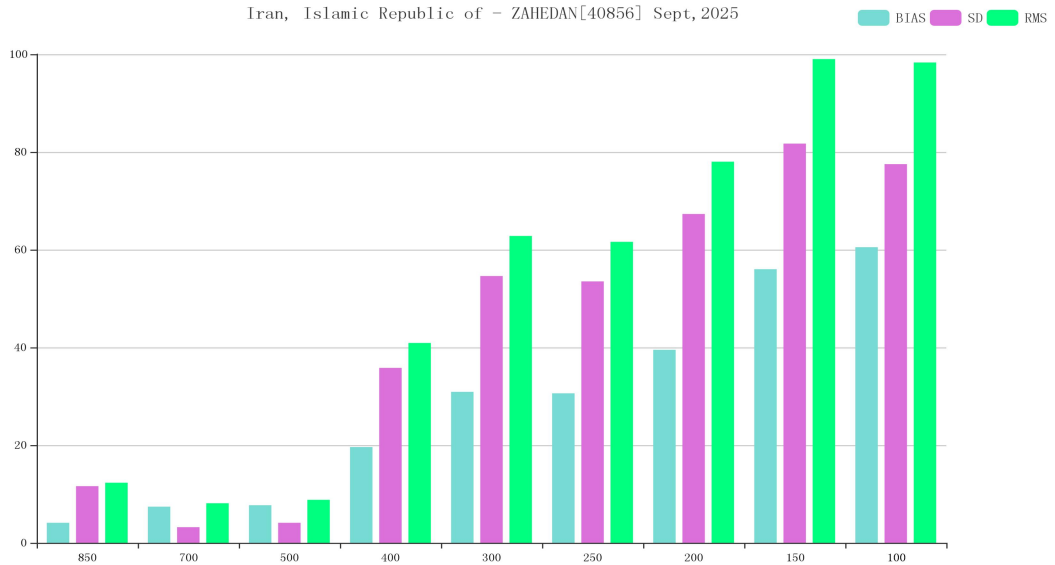
Figure 15 BIAS、SD and RMS of GPH for station 40856*(OBS-TIME:00)
