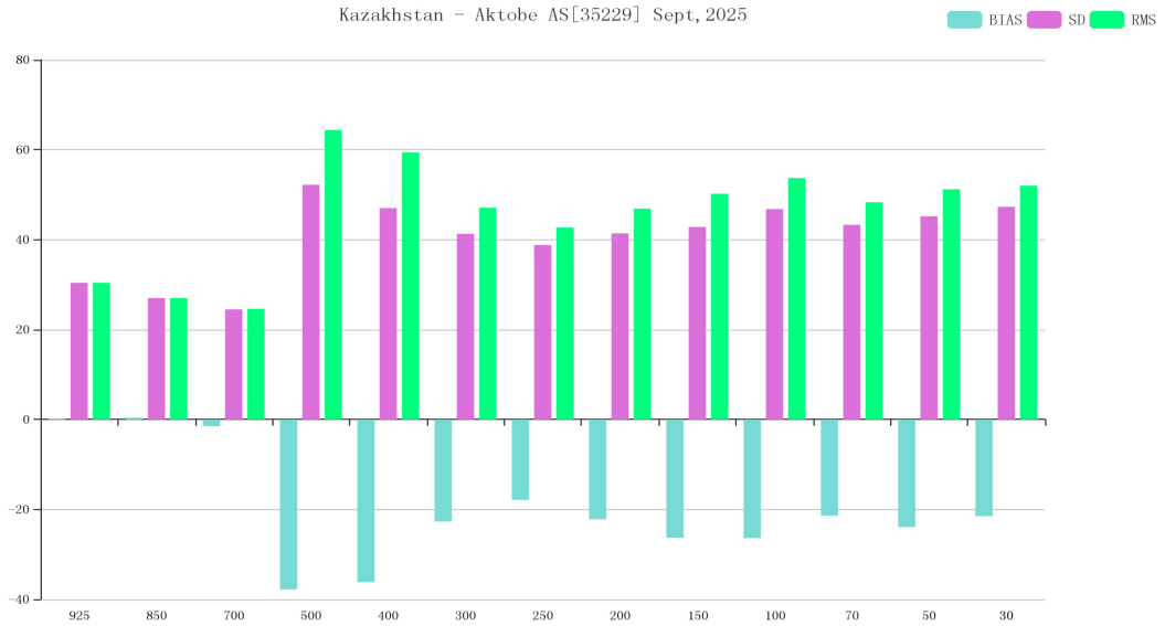
Figure 7 BIAS、SD and RMS of GPH for station 35229*(OBS-TIME:00)
