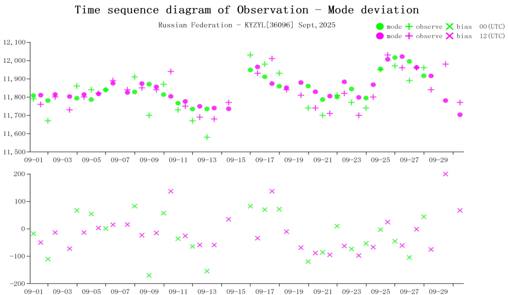
Figure 10 Time-series representation of GPH Obs minus first guess for station 36096*(Level:200)
