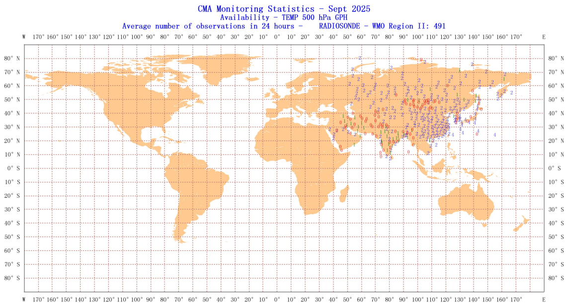
Figure 2 Location of all radiosonde stations reporting geopotential height average number of observations in 24 hours in Region II over the month of September 2025
