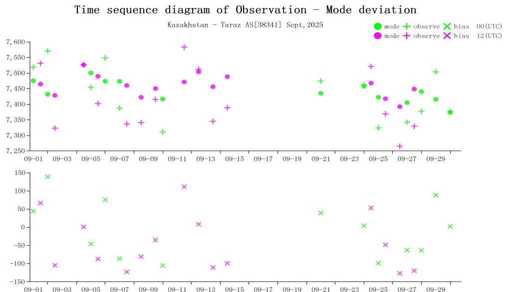
Figure 14 Time-series representation of GPH Obs minus first guess for station 38341*(Level:400)
