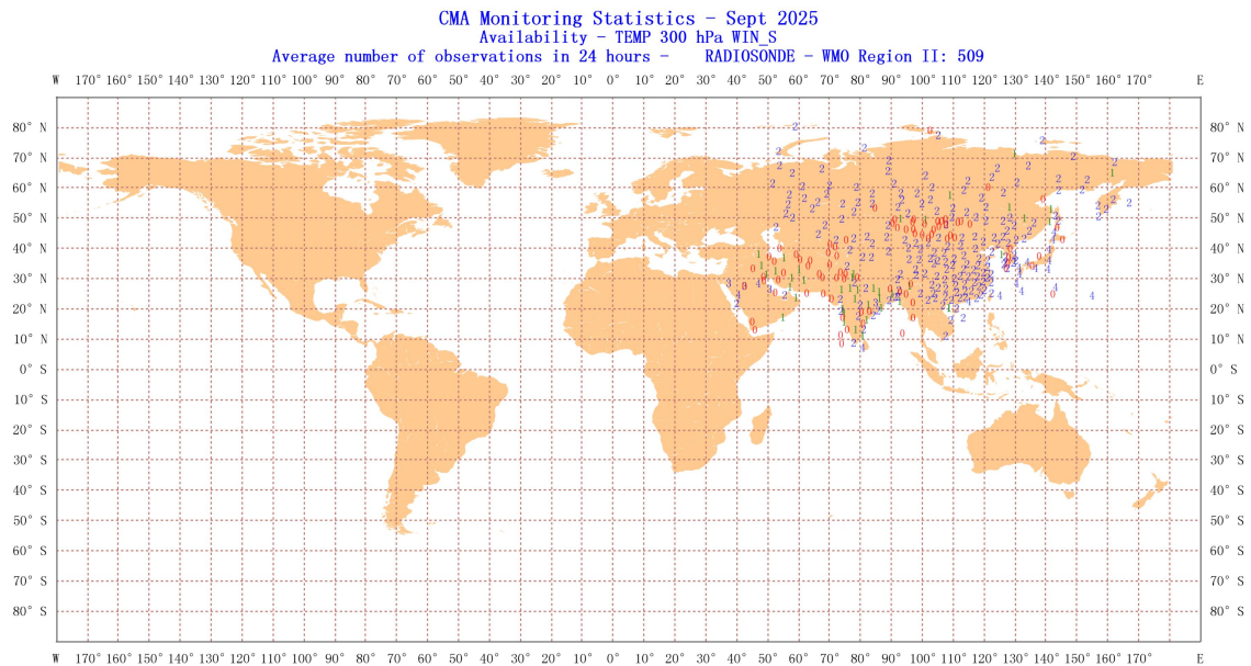
Figure 22 Location of all radiosonde stations reporting vector wind average number of observations in 24 hours in Region II over the month of September 2025
