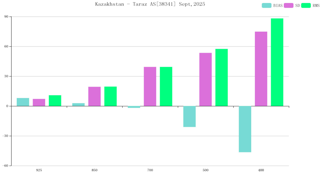
Figure 13 BIAS、SD and RMS of GPH for station 38341*(OBS-TIME:12)
