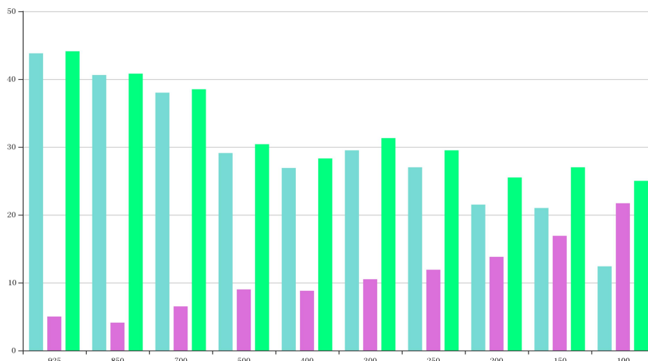
Figure 17 BIAS、SD and RMS of GPH for station 42348(OBS-TIME:00)
