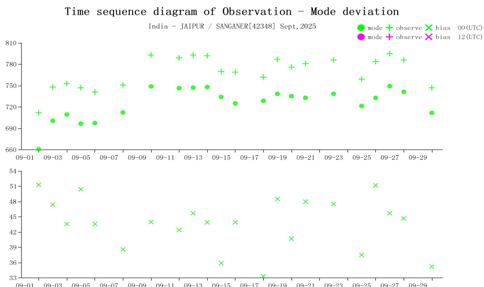
Figure 18 Time-series representation of GPH Obs minus first guess for station 42348(Level:925)
