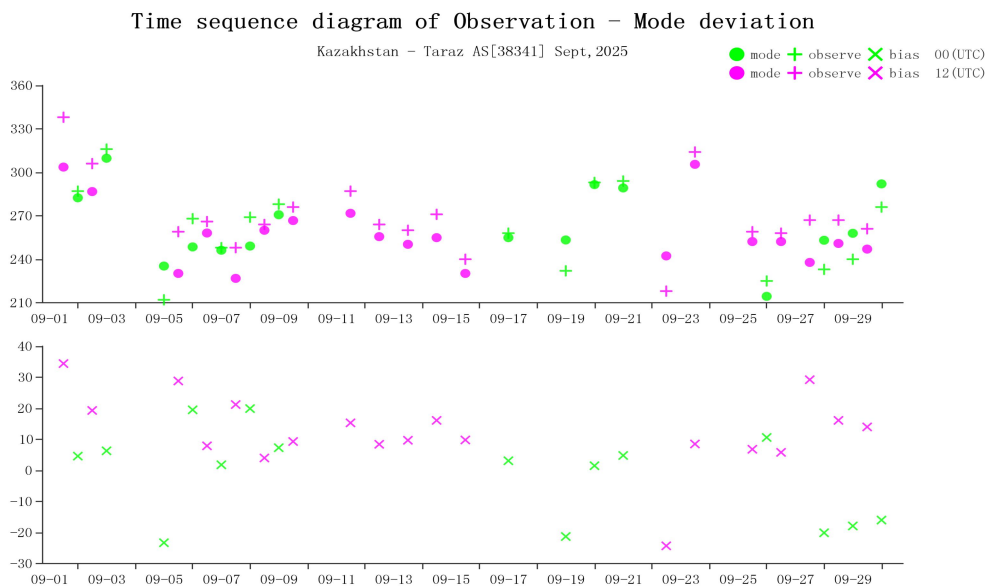
Figure 32 Time-series representation of WIN_D Obs minus first guess for station 38341*(Level:500)
