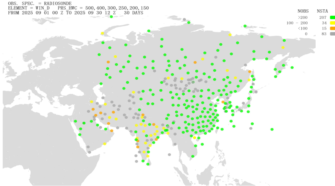
Figure 27 Location of all radiosonde stations reporting wind direction observations in Region II over the month of September 2025. NOBS shows the total number of observations received at RWC-Beijing, corresponding total number of stations (NSTA) and color scale are shown at the top of the figure, color green refers to NOBS is higher than 200, color yellow refers to NOBS is between 100 and 200(including 200), color orange refers to NOBS is between 0 and 100(including 100), and color gray refers to NOBS is 0
