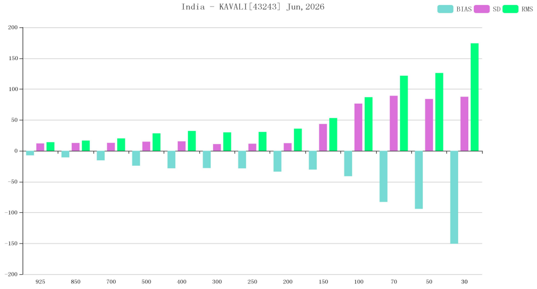
Figure 13 BIAS、SD and RMS of GPH for station 43243(OBS-TIME:00)
