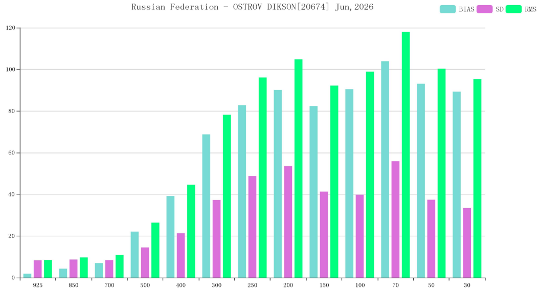
Figure 5 BIAS、SD and RMS of GPH for station 20674*(OBS-TIME:00)
