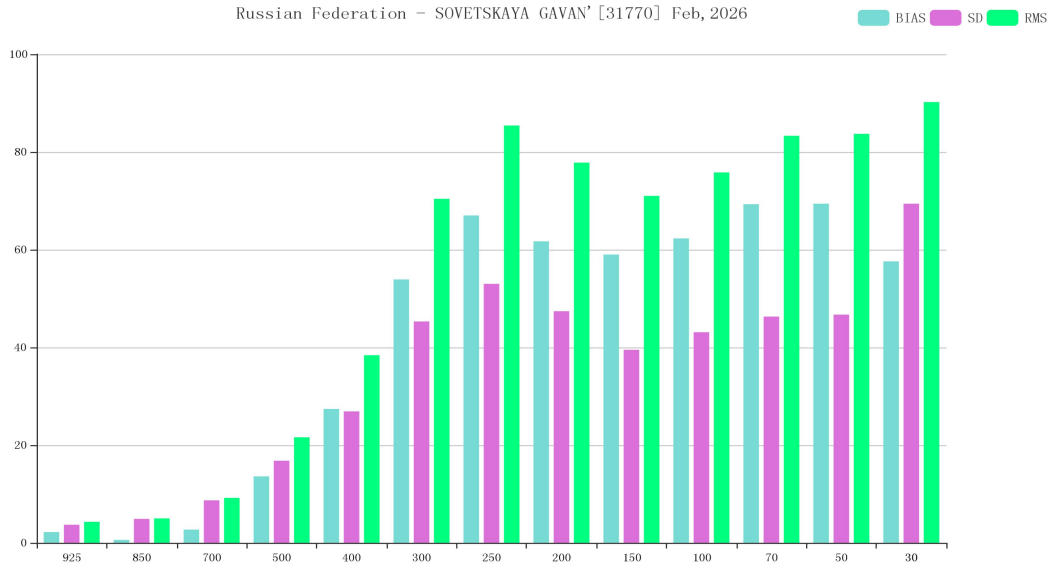
Figure 5 BIAS、SD and RMS of GPH for station 31770*(OBS-TIME:00)
