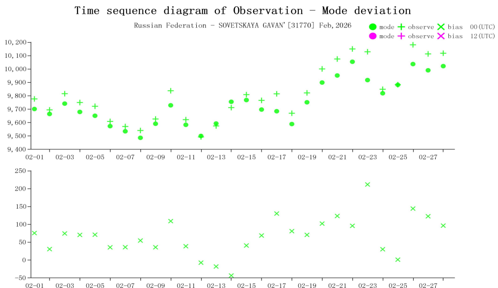
Figure 6 Time-series representation of GPH Obs minus first guess for station 31770*(Level:250)
