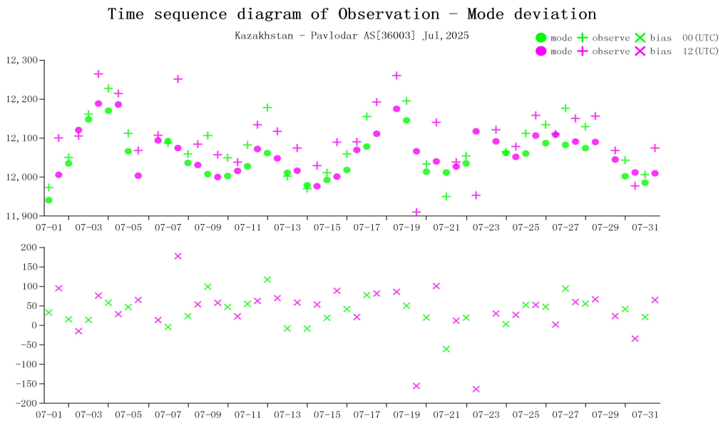
Figure 14 Time-series representation of GPH Obs minus first guess for station 36003*(Level:200)
