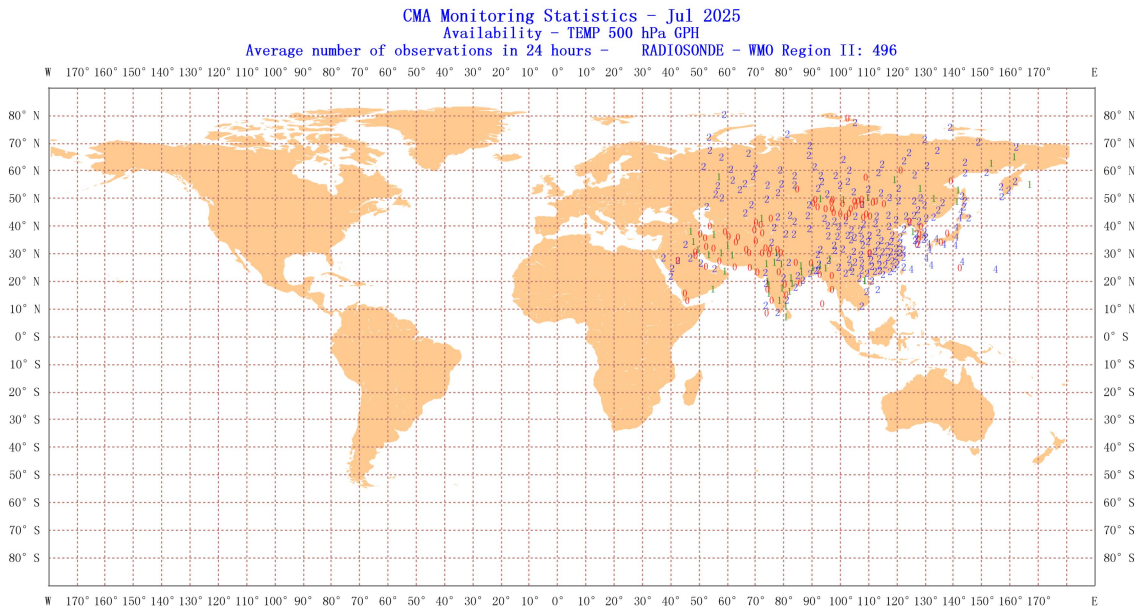
Figure 2 Location of all radiosonde stations reporting geopotential height average number of observations in 24 hours in Region II over the month of July 2025
