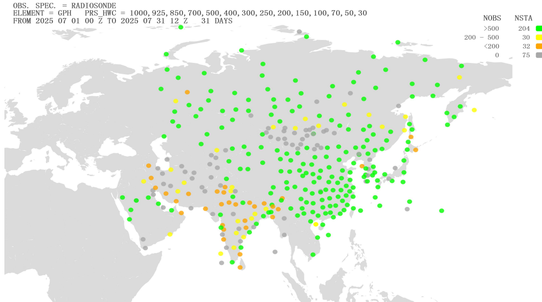
Figure 1 Location of all radiosonde stations reporting geopotential height observations in Region II over the month of July 2025. NOBS shows the total number of observations received at RWC-Beijing, corresponding total number of stations (NSTA) and color scale are shown at the top of the figure, color green refers to NOBS is higher than 500, color yellow refers to NOBS is between 200 and 500(including 500), color orange refers to NOBS is between 0 and 200(including 200), and color gray refers to NOBS is 0
