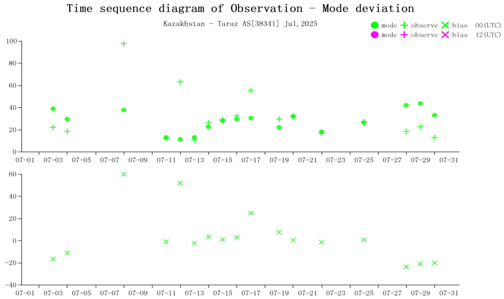
Figure 30 Time-series representation of WIN_S Obs minus first guess for station 38341*(Level:250)
