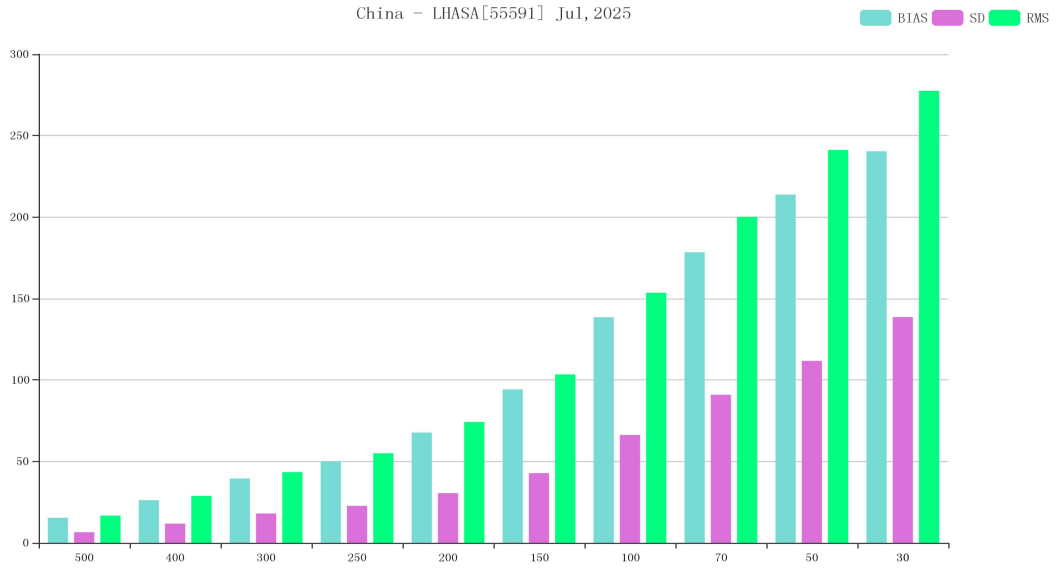
Figure 23 BIAS、SD and RMS of GPH for station 55591(OBS-TIME:12)
