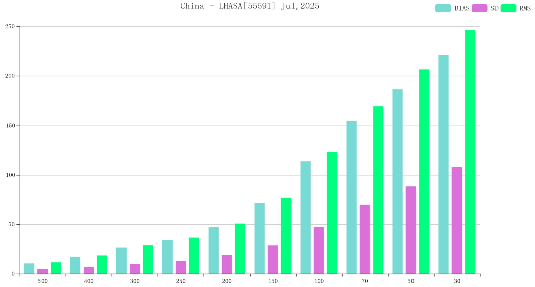
Figure 21 BIAS、SD and RMS of GPH for station 55591(OBS-TIME:00)
