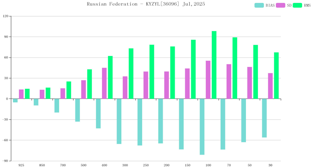
Figure 15 BIAS、SD and RMS of GPH for station 36096*(OBS-TIME:00)
