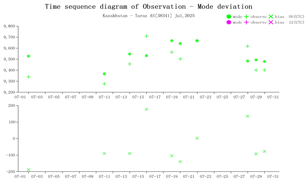
Figure 18 Time-series representation of GPH Obs minus first guess for station 38341*(Level:300)
