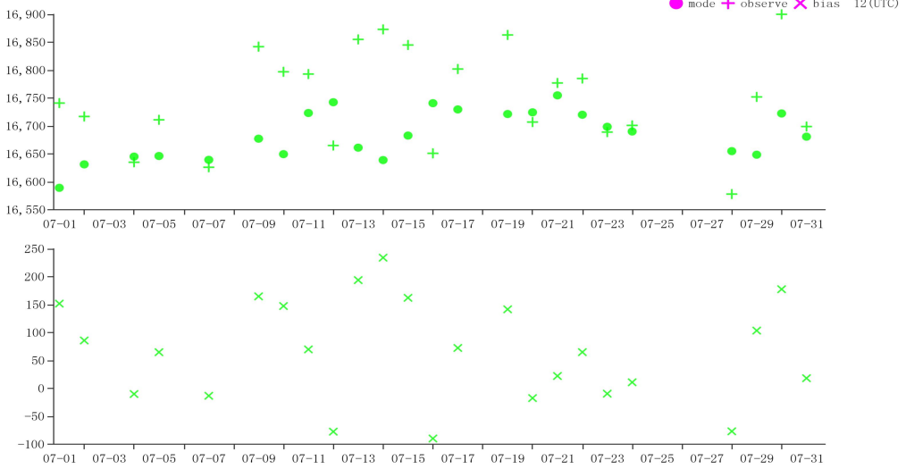
Figure 12 Time-series representation of GPH Obs minus first guess for station 31770*(Level:100)
