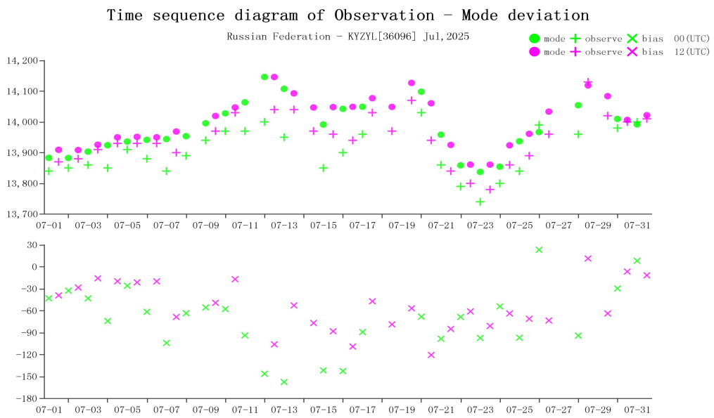
Figure 16 Time-series representation of GPH Obs minus first guess for station 36096*(Level:150)
