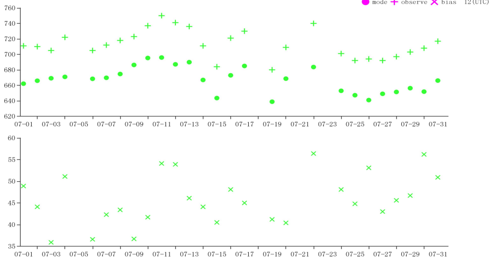
Figure 20 Time-series representation of GPH Obs minus first guess for station 42348(Level:925)
