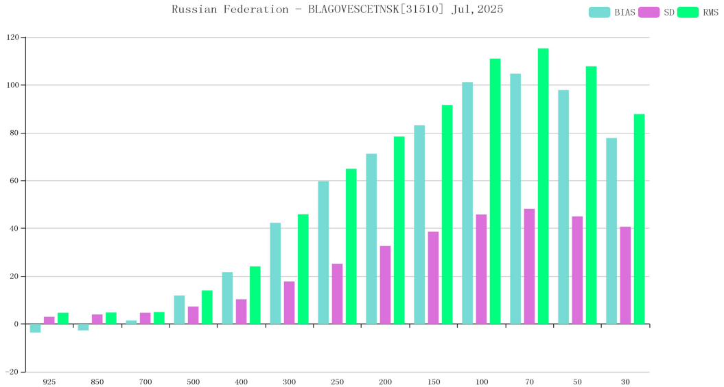
Figure 9 BIAS、SD and RMS of GPH for station 31510*(OBS-TIME:00)
