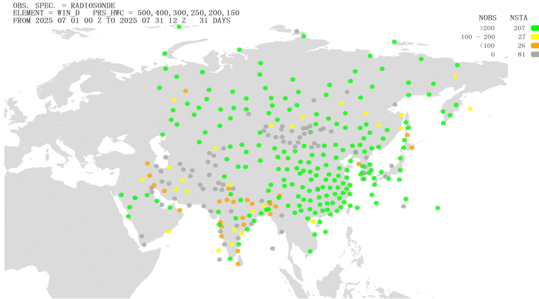
Figure 31 Location of all radiosonde stations reporting wind direction observations in Region II over the month of July 2025. NOBS shows the total number of observations received at RWC-Beijing, corresponding total number of stations (NSTA) and color scale are shown at the top of the figure, color green refers to NOBS is higher than 200, color yellow refers to NOBS is between 100 and 200(including 200), color orange refers to NOBS is between 0 and 100(including 100), and color gray refers to NOBS is 0
