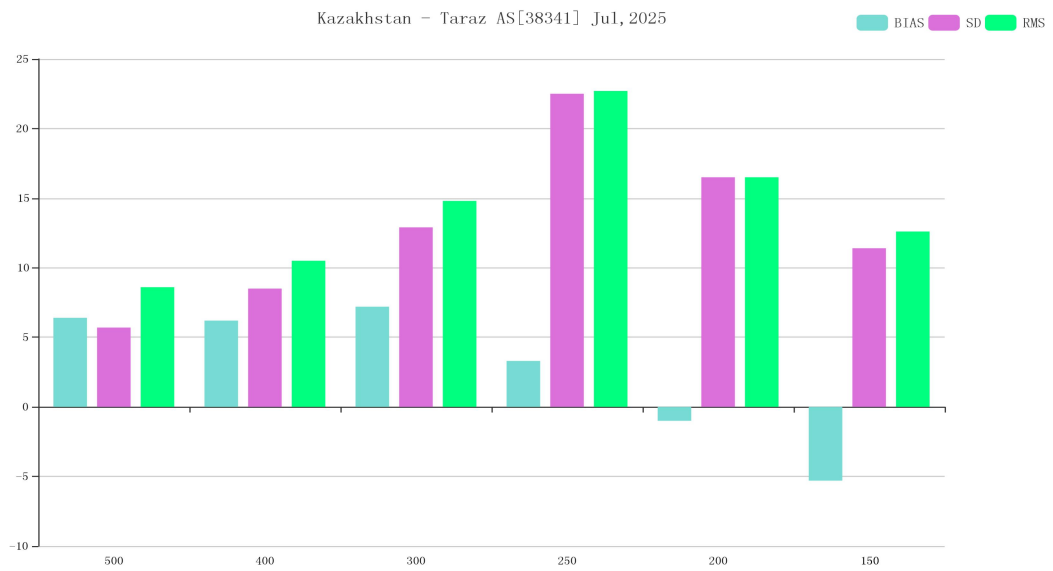
Figure 29 BIAS、SD and RMS of WIN_S for station 38341*(OBS-TIME:00)
