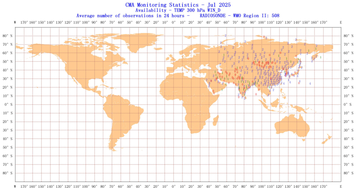
Figure 32 Location of all radiosonde stations reporting wind direction average number of observations in 24 hours in Region II over the month of July 2025
