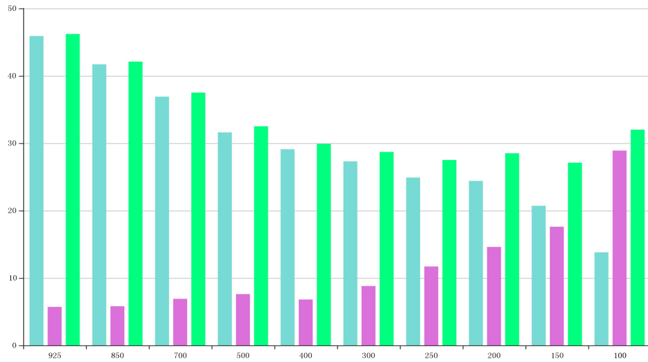
Figure 19 BIAS、SD and RMS of GPH for station 42348(OBS-TIME:00)
