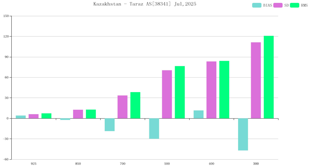
Figure 17 BIAS、SD and RMS of GPH for station 38341*(OBS-TIME:00)
