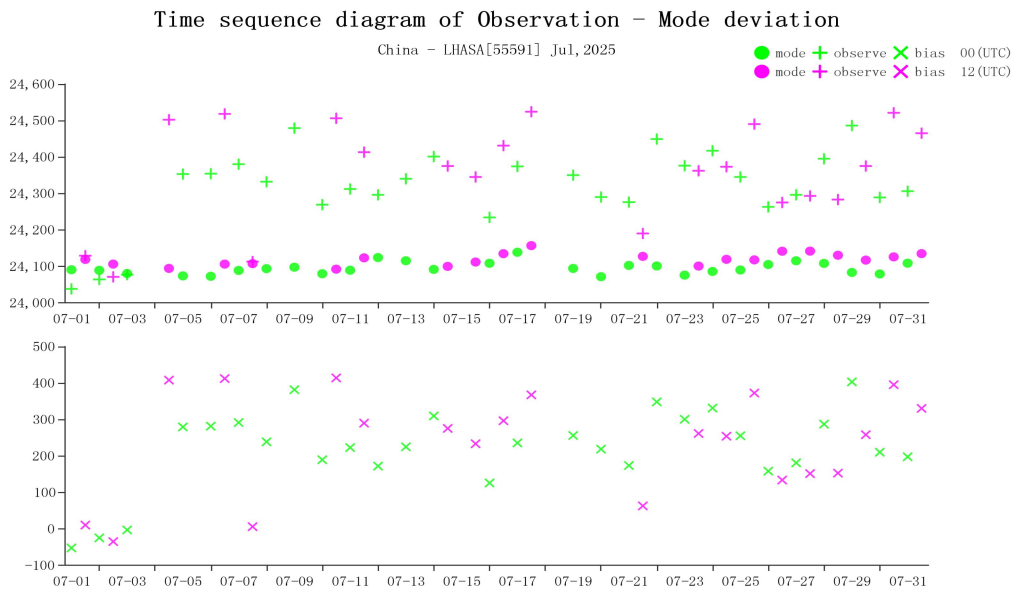
Figure 22 Time-series representation of GPH Obs minus first guess for station 55591(Level:30)
