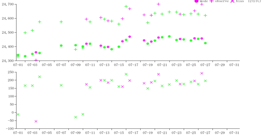
Figure 6 Time-series representation of GPH Obs minus first guess for station 25913*(Level:30)
