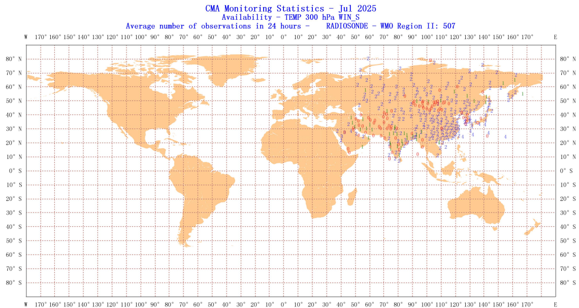
Figure 26 Location of all radiosonde stations reporting vector wind average number of observations in 24 hours in Region II over the month of July 2025
