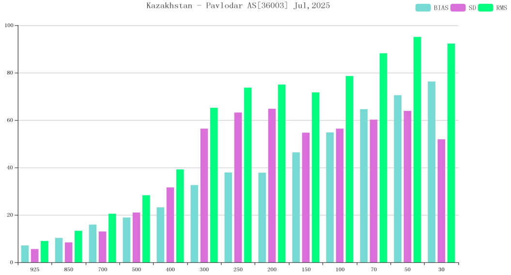
Figure 13 BIAS、SD and RMS of GPH for station 36003*(OBS-TIME:12)
