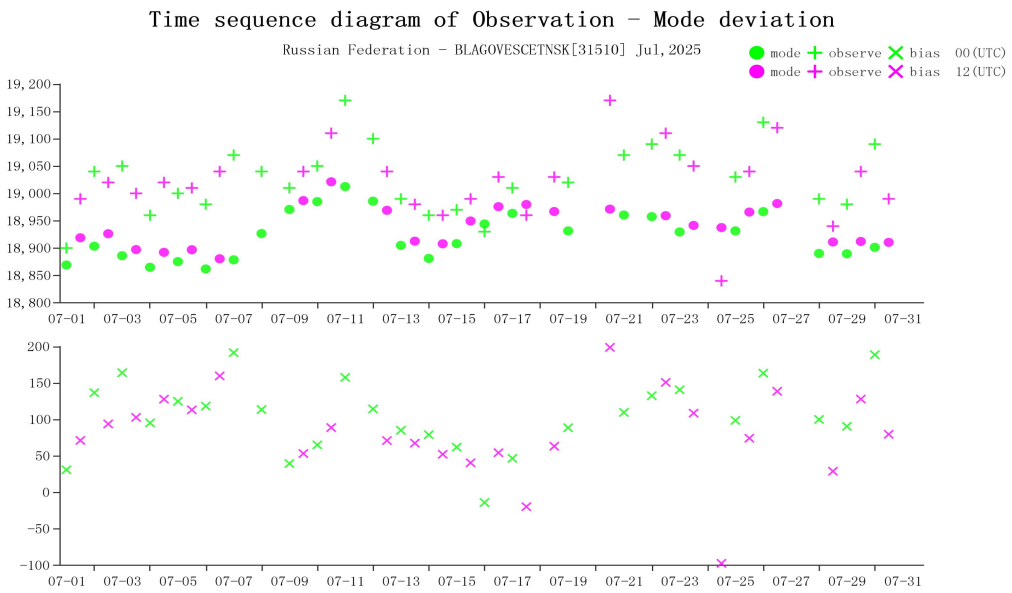
Figure 10 Time-series representation of GPH Obs minus first guess for station 31510*(Level:70)
