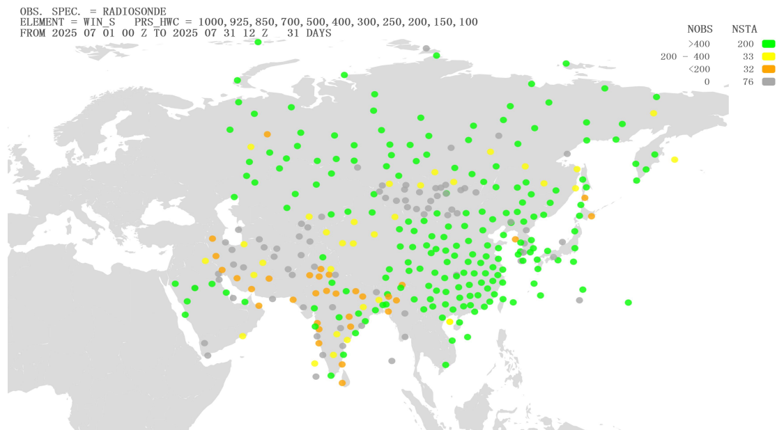
Figure 25 Location of all radiosonde stations reporting vector wind observations in Region II over the month of July 2025. NOBS shows the total number of observations received at RWC-Beijing, corresponding total number of stations (NSTA) and color scale are shown at the top of the figure, color green refers to NOBS is higher than 400, color yellow refers to NOBS is between 200 and 400(including 400), color orange refers to NOBS is between 0 and 200(including 200), and color gray refers to NOBS is 0
