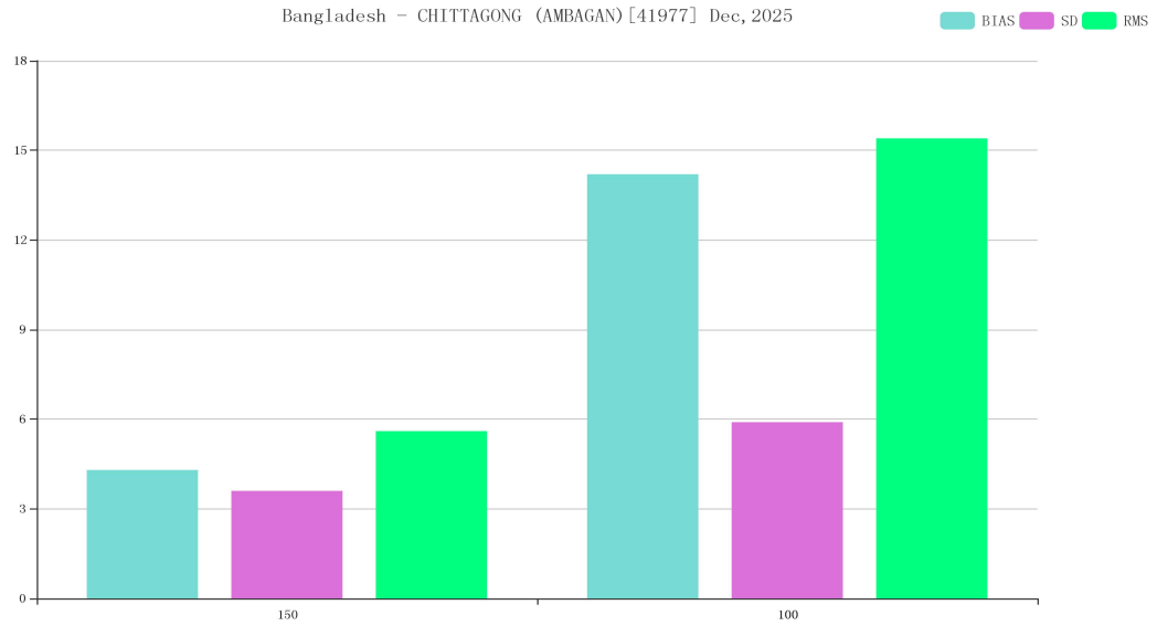
Figure 11 BIAS、SD and RMS of WIN_S for station 41977(OBS-TIME:00)
