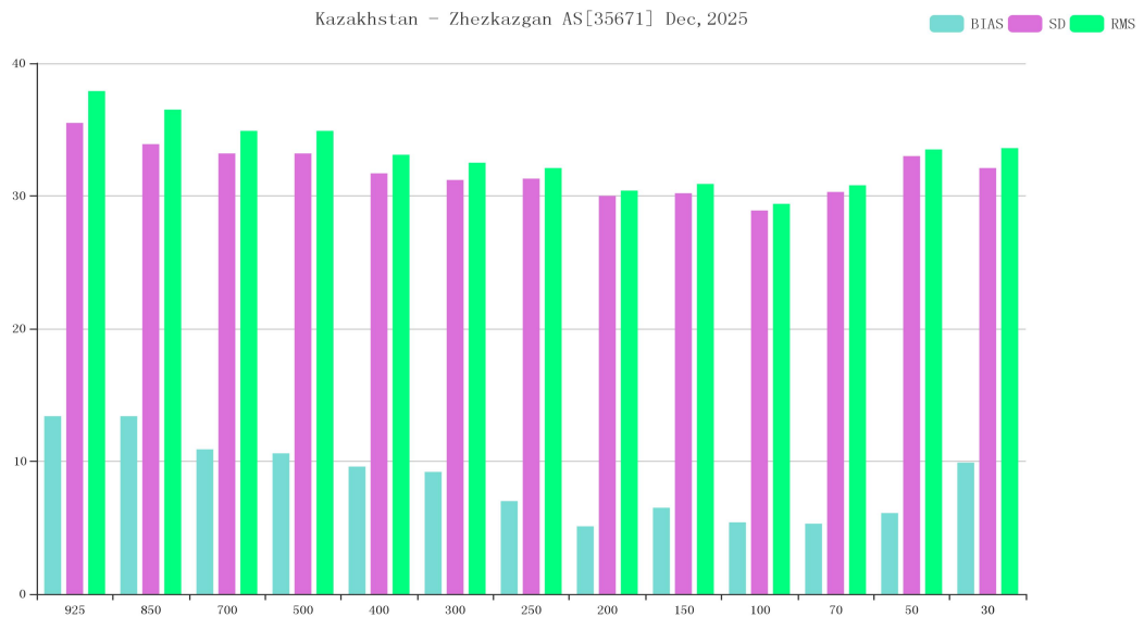
Figure 5 BIAS、SD and RMS of GPH for station 35671*(OBS-TIME:00)
