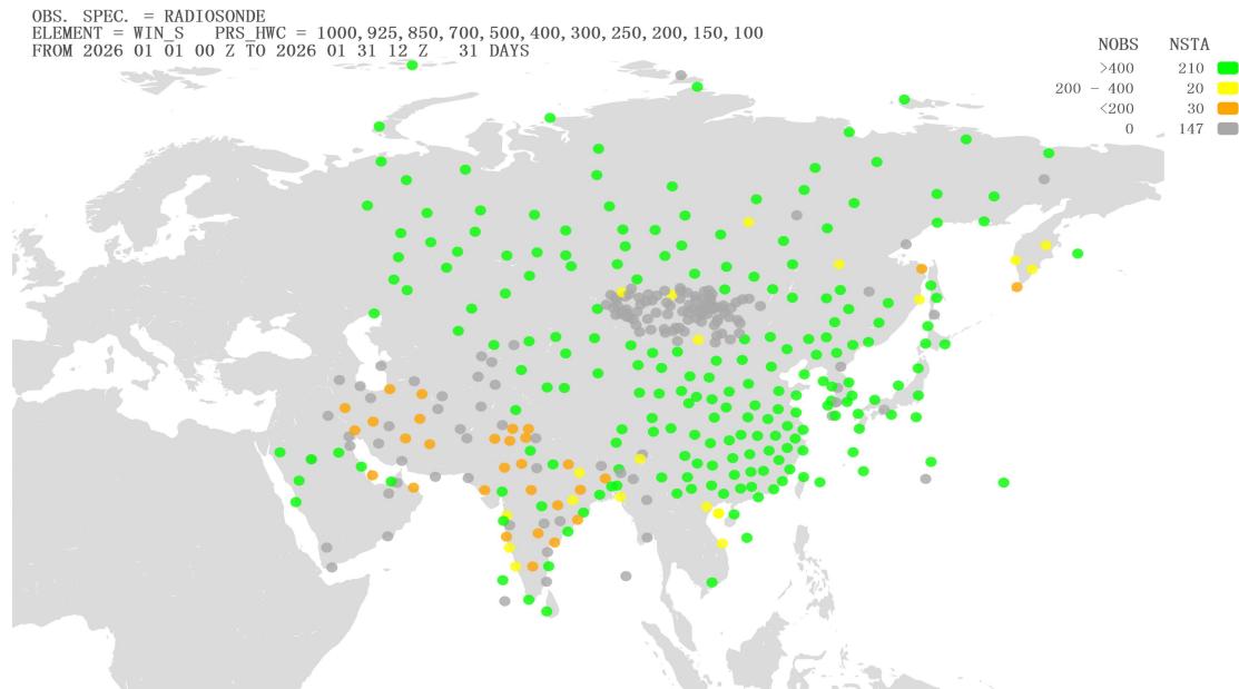
Figure 9 Location of all radiosonde stations reporting vector wind observations in Region II over the month of January 2026. NOBS shows the total number of observations received at RWC-Beijing, corresponding total number of stations (NSTA) and color scale are shown at the top of the figure, color green refers to NOBS is higher than 400, color yellow refers to NOBS is between 200 and 400(including 400), color orange refers to NOBS is between 0 and 200(including 200), and color grey refers to NOBS is 0
