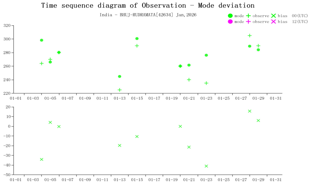
Figure 16 Time-series representation of WIN_D Obs minus first guess for station 42634(Level:500)
