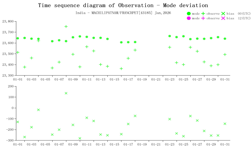
Figure 8 Time-series representation of GPH Obs minus first guess for station 43185(Level:30)
