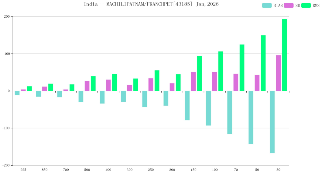
Figure 7 BIAS、SD and RMS of GPH for station 43185(OBS-TIME:00)
