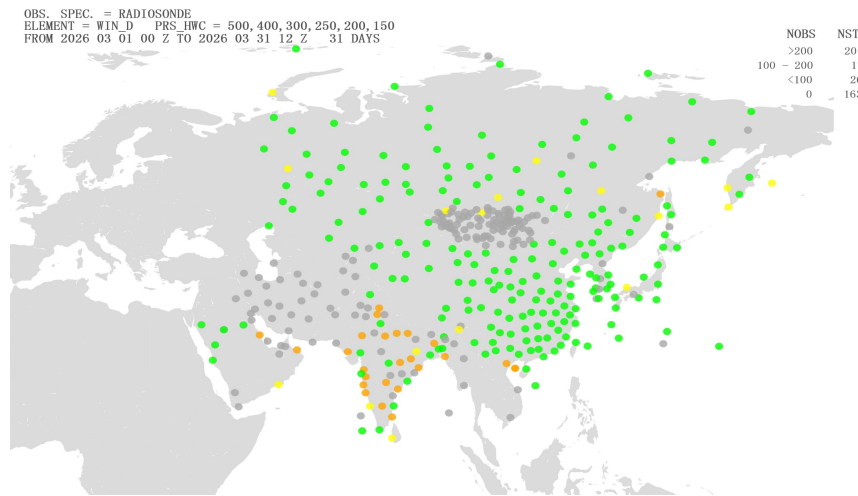
Figure 5 Location of all radiosonde stations reporting wind direction observations in Region II over the month of March 2026. NOBS shows the total number of observations received at RWC-Beijing, corresponding total number of stations (NSTA) and color scale are shown at the top of the figure, color green refers to NOBS is higher than 200, color yellow refers to NOBS is between 100 and 200(including 200), color orange refers to NOBS is between 0 and 100(including 100), and color gray refers to NOBS is 0
