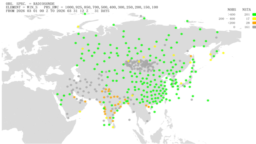
Figure 3 Location of all radiosonde stations reporting vector wind observations in Region II over the month of March 2026. NOBS shows the total number of observations received at RWC-Beijing, corresponding total number of stations (NSTA) and color scale are shown at the top of the figure, color green refers to NOBS is higher than 400, color yellow refers to NOBS is between 200 and 400(including 400), color orange refers to NOBS is between 0 and 200(including 200), and color gray refers to NOBS is 0
