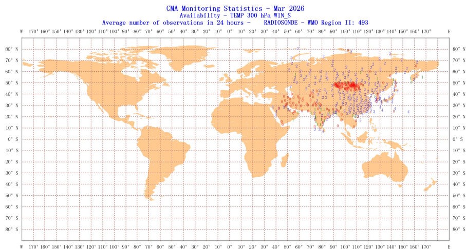
Figure 4 Location of all radiosonde stations reporting vector wind average number of observations in 24 hours in Region II over the month of March 2026
