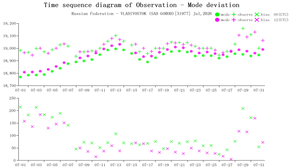
Figure 18 Time-series representation of GPH Obs minus first guess for station 31977*(Level:70)
