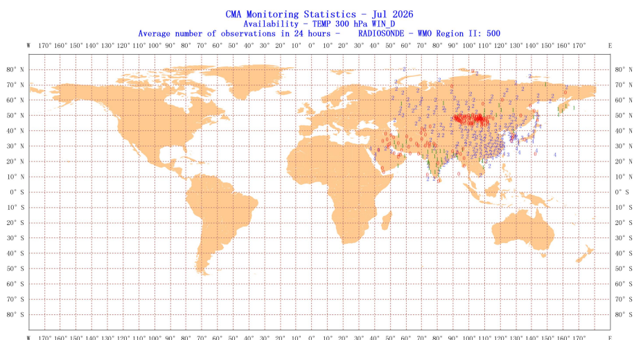
Figure 32 Location of all radiosonde stations reporting wind direction average number of observations in 24 hours in Region II over the month of July 2026
