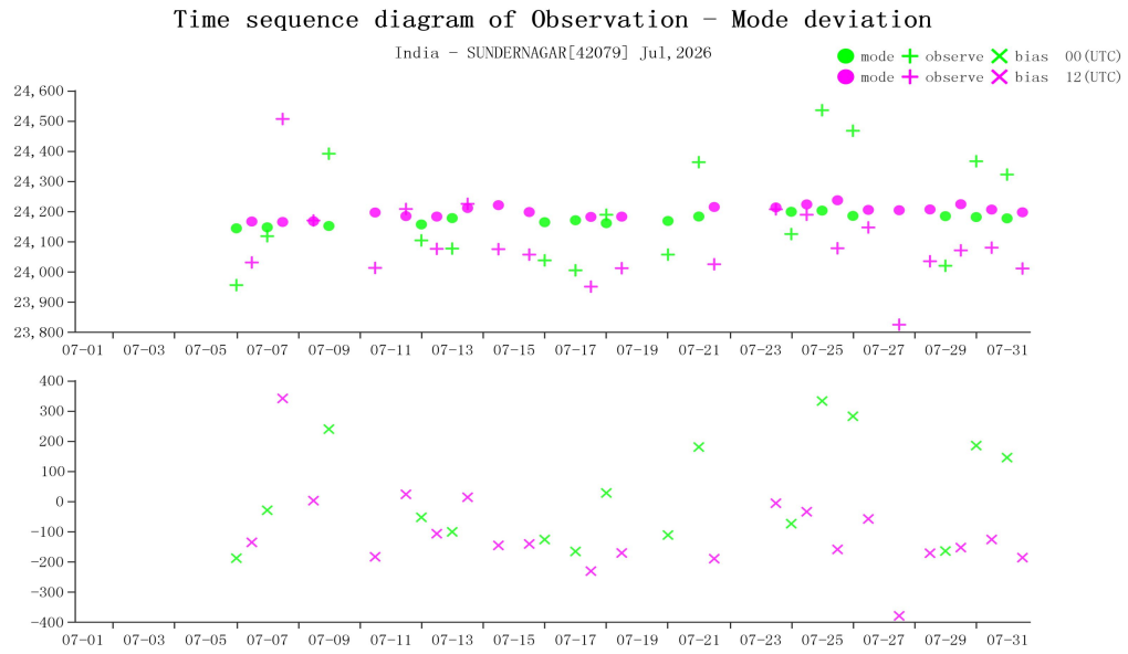
Figure 20 Time-series representation of GPH Obs minus first guess for station 42079(Level:30)
