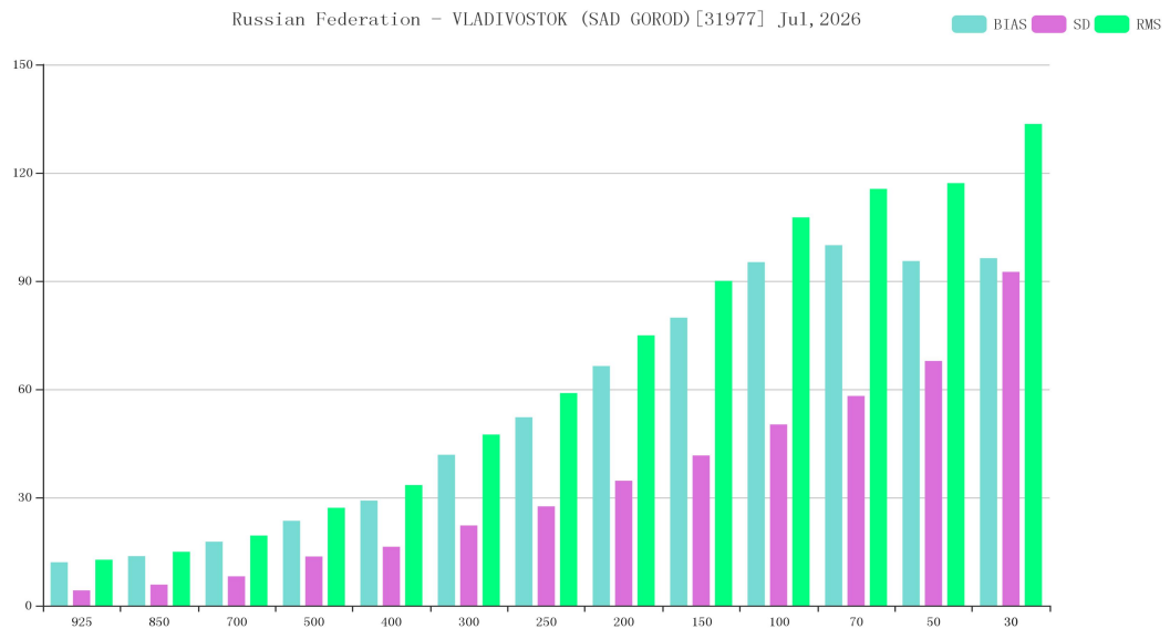
Figure 17 BIAS、SD and RMS of GPH for station 31977*(OBS-TIME:00)
