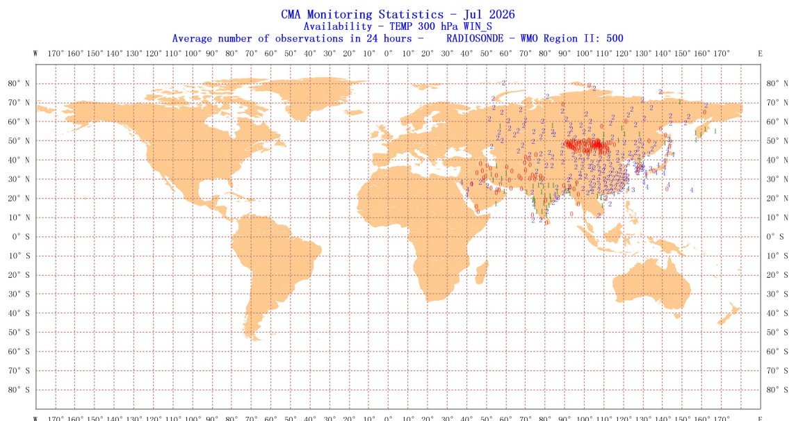
Figure 30 Location of all radiosonde stations reporting vector wind average number of observations in 24 hours in Region II over the month of July 2026
