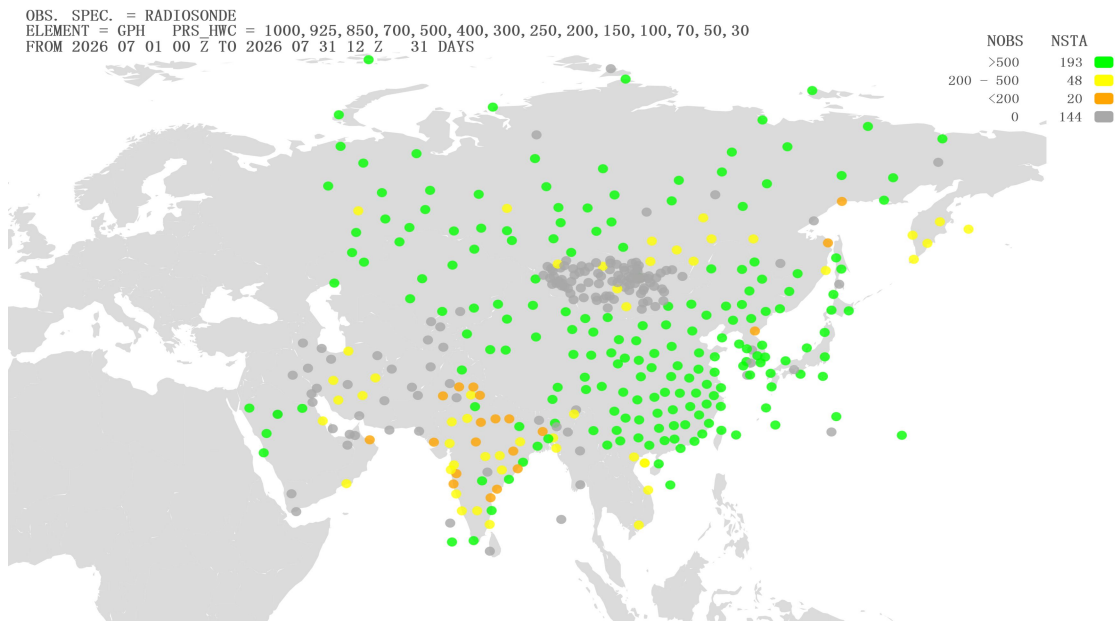
Figure 1 Location of all radiosonde stations reporting geopotential height observations in Region II over the month of July 2026. NOBS shows the total number of observations received at RWC-Beijing, corresponding total number of stations (NSTA) and color scale are shown at the top of the figure, color green refers to NOBS is higher than 500, color yellow refers to NOBS is between 200 and 500(including 500), color orange refers to NOBS is between 0 and 200(including 200), and color gray refers to NOBS is 0
