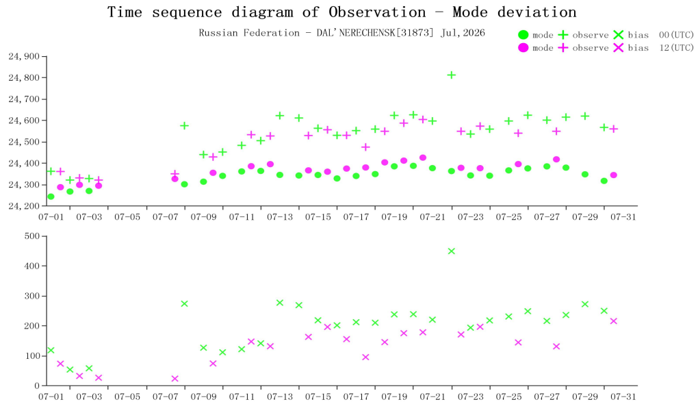
Figure 14 Time-series representation of GPH Obs minus first guess for station 31873*(Level:30)
