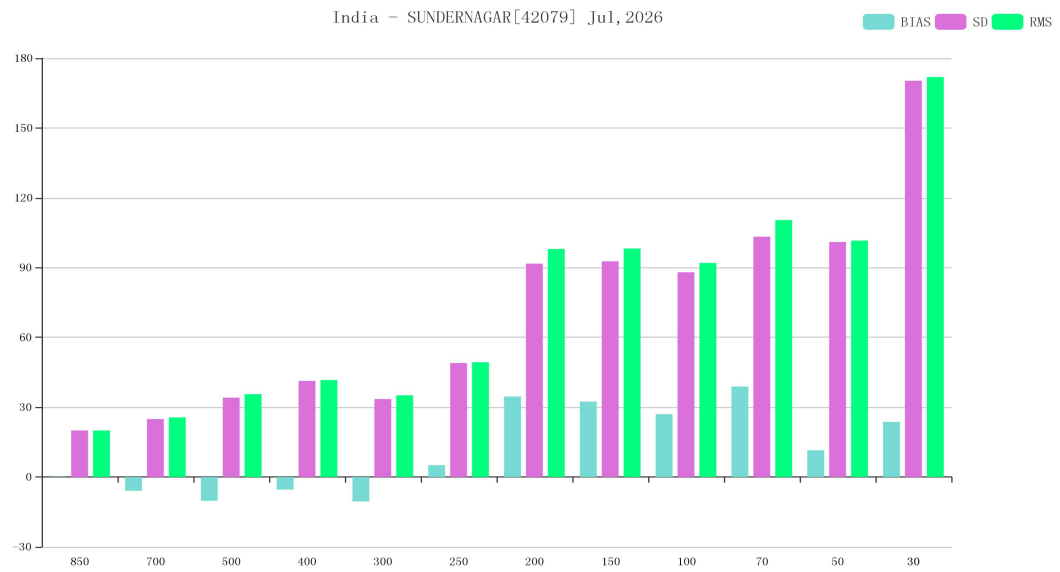
Figure 19 BIAS、SD and RMS of GPH for station 42079(OBS-TIME:00)
