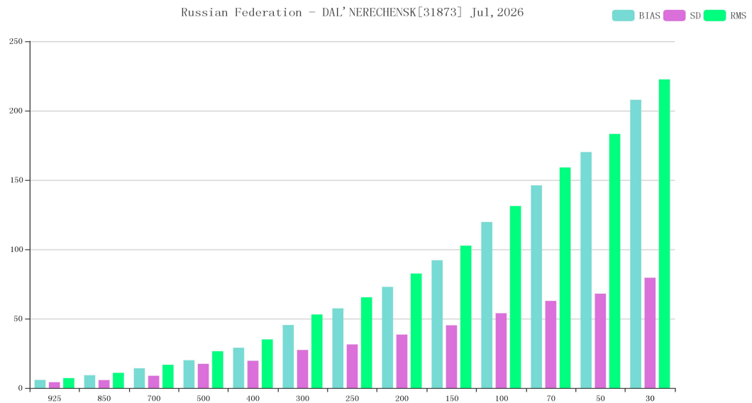
Figure 13 BIAS、SD and RMS of GPH for station 31873*(OBS-TIME:00)
