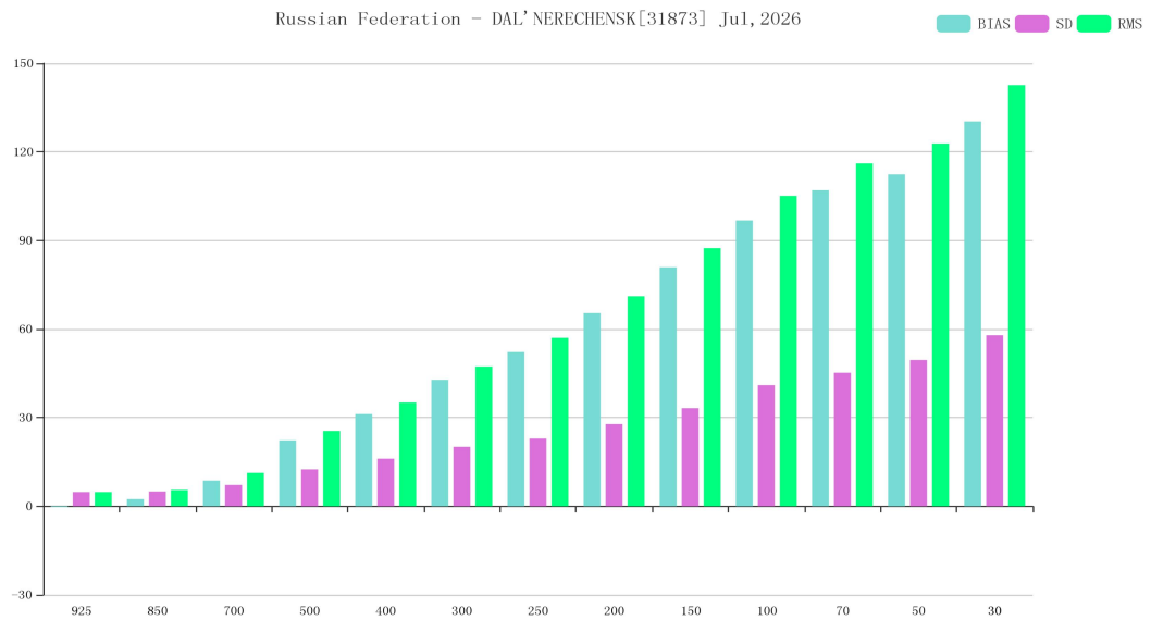
Figure 15 BIAS、SD and RMS of GPH for station 31873*(OBS-TIME:12)
