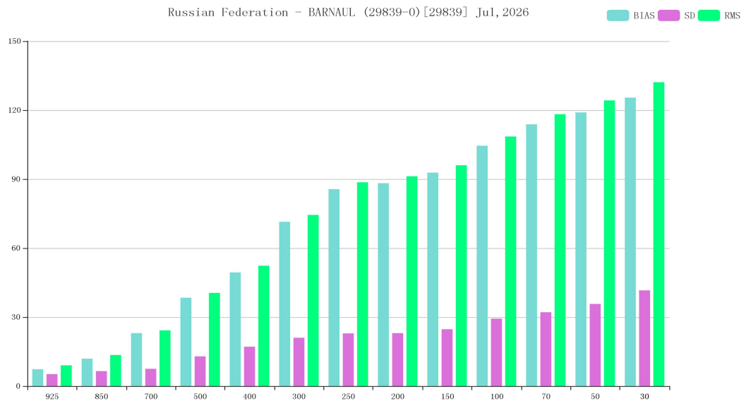
Figure 11 BIAS、SD and RMS of GPH for station 29839*(OBS-TIME:12)
