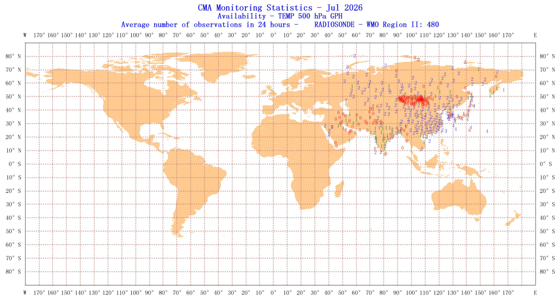
Figure 2 Location of all radiosonde stations reporting geopotential height average number of observations in 24 hours in Region II over the month of July 2026
