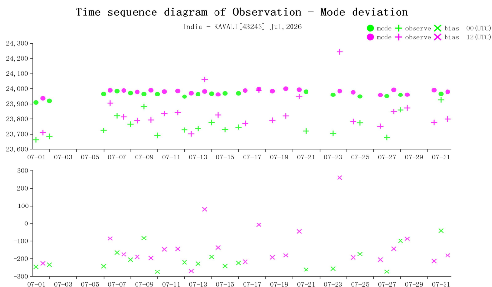
Figure 26 Time-series representation of GPH Obs minus first guess for station 43243(Level:30)
