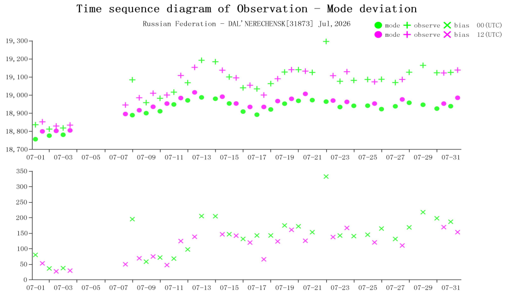
Figure 16 Time-series representation of GPH Obs minus first guess for station 31873*(Level:70)
