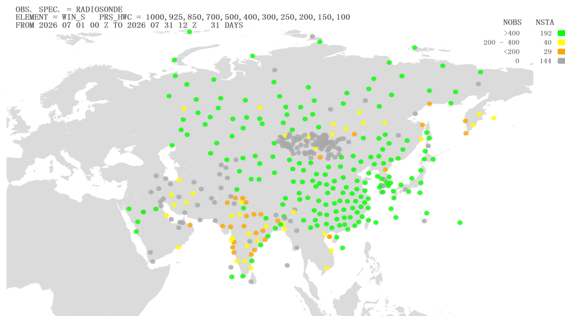
Figure 29 Location of all radiosonde stations reporting vector wind observations in Region II over the month of July 2026. NOBS shows the total number of observations received at RWC-Beijing, corresponding total number of stations (NSTA) and color scale are shown at the top of the figure, color green refers to NOBS is higher than 400, color yellow refers to NOBS is between 200 and 400(including 400), color orange refers to NOBS is between 0 and 200(including 200), and color gray refers to NOBS is 0
