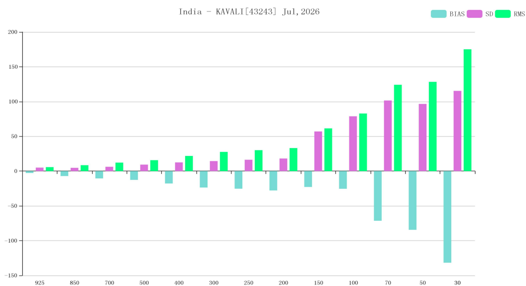
Figure 25 BIAS、SD and RMS of GPH for station 43243(OBS-TIME:12)
