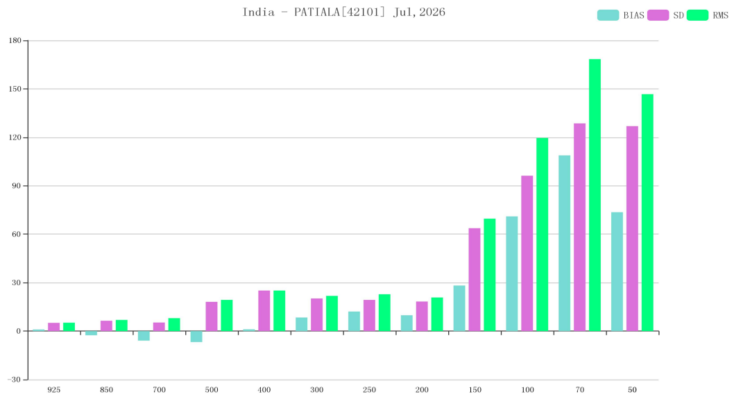
Figure 21 BIAS、SD and RMS of GPH for station 42101*(OBS-TIME:00)
