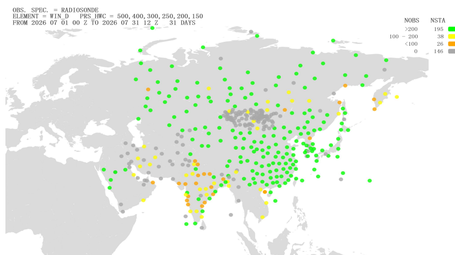
Figure 31 Location of all radiosonde stations reporting wind direction observations in Region II over the month of July 2026. NOBS shows the total number of observations received at RWC-Beijing, corresponding total number of stations (NSTA) and color scale are shown at the top of the figure, color green refers to NOBS is higher than 200, color yellow refers to NOBS is between 100 and 200(including 200), color orange refers to NOBS is between 0 and 100(including 100), and color gray refers to NOBS is 0
