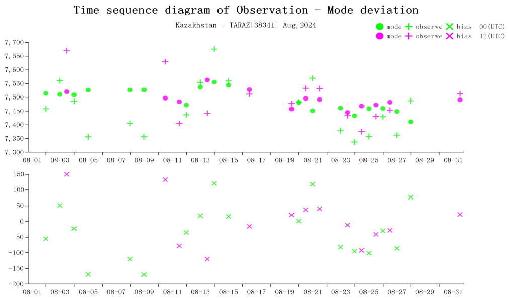
Time-series representation of GPH Obs minus first guess for station 38341(Level:400)
