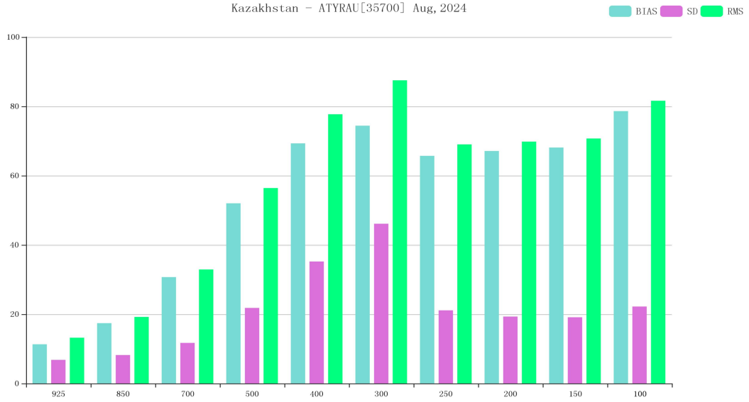
BIAS、SD and RMS of GPH for station 35700(OBS-TIME:12)
