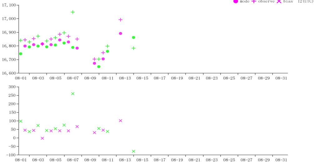
Time-series representation of GPH Obs minus first guess for station 32150(Level:100)
