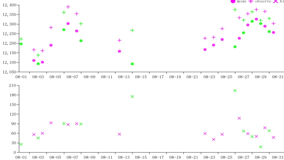
Time-series representation of GPH Obs minus first guess for station 35700(Level:200)
